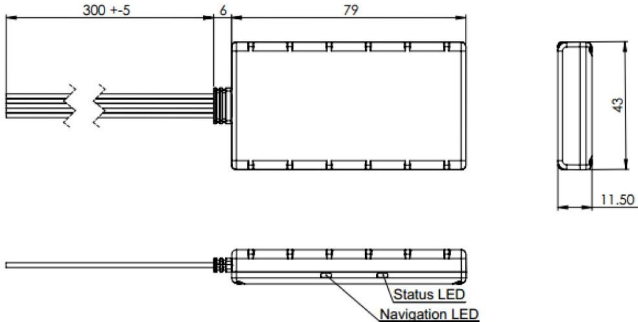
Figure 1 FMB9YX view & dimensions (tolerance ±2mm)
